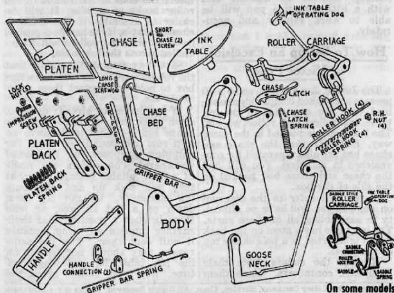
Press parts and their names
